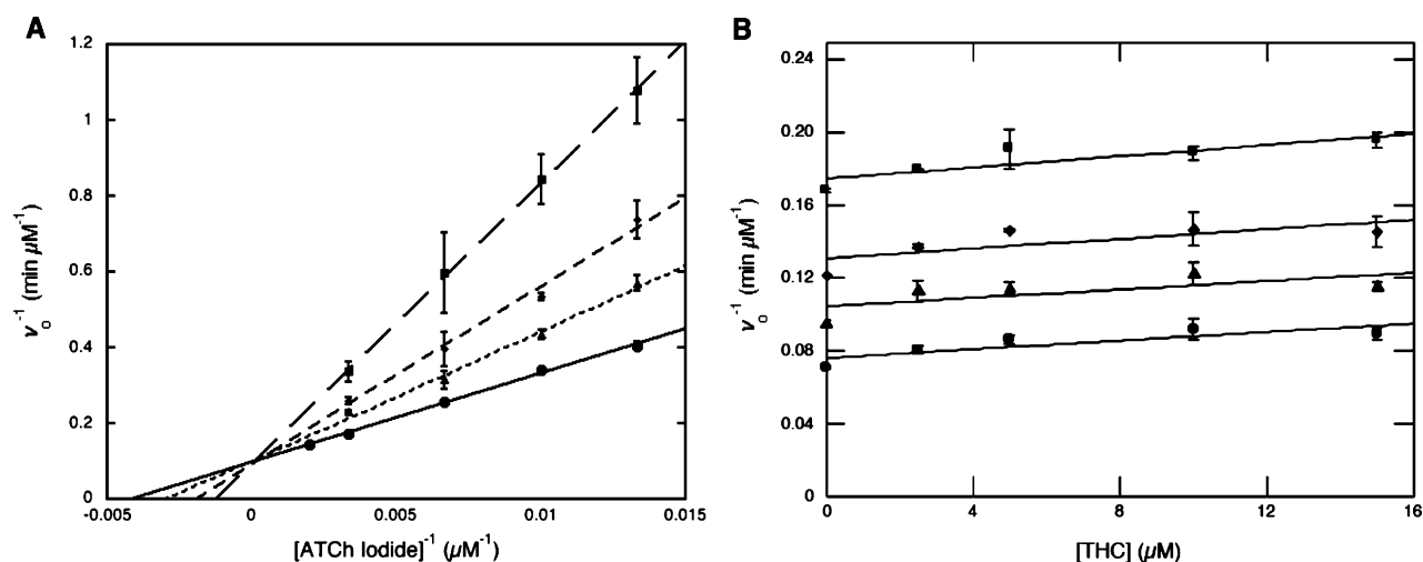
Figure 3. (A) Kinetic analysis of AChE inhibition by THC: 0 (●), 6.25 (▲), 12.5 (◆), and 25.0 \mu\text{M} (■). Steady-state kinetic analysis was performed using acetylthiocholine (75–300 \mu\text{M} ) and Ellman's reagent (340 \mu\text{M} ) at 37 °C. (B) Dixon plots of 1/v versus [THC] at different fixed concentrations of propidium iodide: 0 (●), 6.25 (▲), 12.5 (◆), and 25 \mu\text{M} (■).
