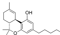
Figure 1. Chemical structure of \Delta^9 -tetrahydrocannabinol (THC).
